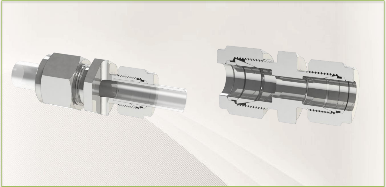
-T-LOCK - TUBE TO TUBE
