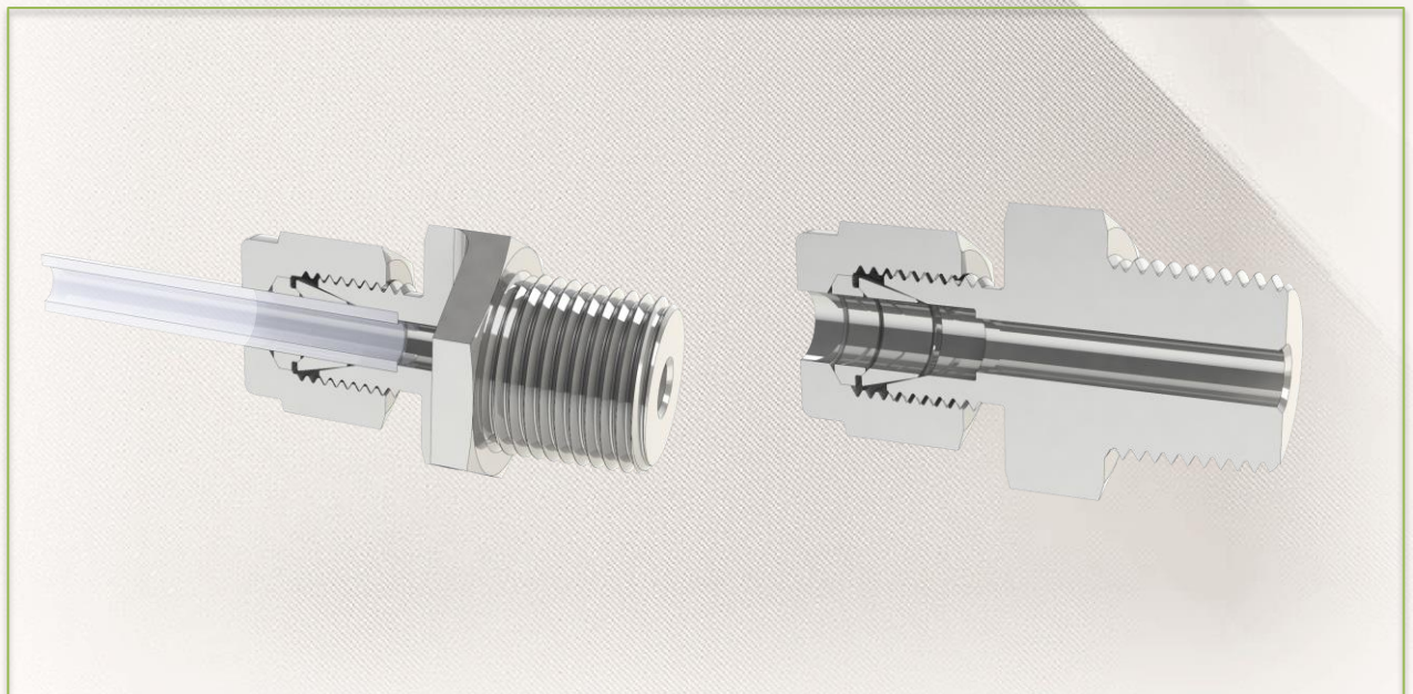
-T-LOCK - THREAD TO TUBE
